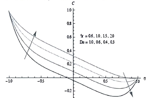
Fig. 6d Variation of Concentration(C) with Sr & Du M=0.5, A_1=1.01, \gamma=0.5, Rd=0.5, \Delta=1, \Delta p=1, Q_1=0.5
