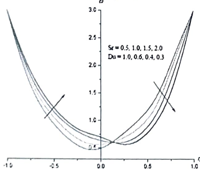
Fig. 6a Variation of axial velocity( f ) with Sr & Du M=0.5, A_1=1.01, \gamma=0.5, Rd=0.5, \Delta=1, \Delta p=1, Q_1=0.5
