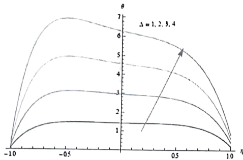
Fig. 3c Variation of temperature( \theta ) with \Delta M=0.5, A1=1.01, Sr=0.6, Du=0.1, \gamma=0.5, Rd=0.5, \Delta p=1, Q1=0.5
