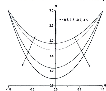
Fig. 7b Variation of micro-rotation( \omega ) with \gamma M=0.5, A_1=1.01, Sr=0.6, Du=0.1, Rd=0.5, \Delta=1, \Delta p=1, Q_1=0.5
