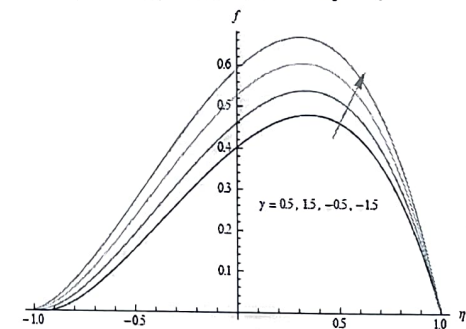
Fig. 7a Variation of axial velocity( f ) with \gamma M=0.5, A_1=1.01, Sr=0.6, Du=0.1, Rd=0.5, \Delta=1, \Delta p=1, Q_1=0.5
