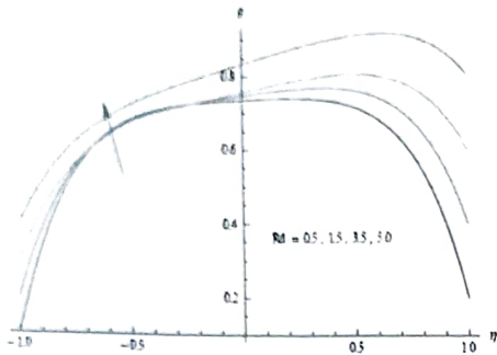
Fig. 5c Variation of temperature( \theta ) with Rd M=0.5, A_1=1.01, Sr=0.6, Du=0.1, \gamma=0.5, \Delta=1, \Delta p=1, Q_1=0.5
