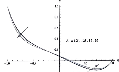
Fig. 4d Variation of Concentration ( C ) with A1 M=0.5, Sr=0.6, Du=0.1, \gamma=0.5, Rd=0.5, \Delta=1, \Delta p=1, Q1=0.5
